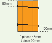
Detail D
